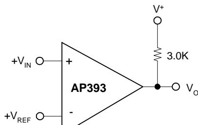
Basic Comparator
