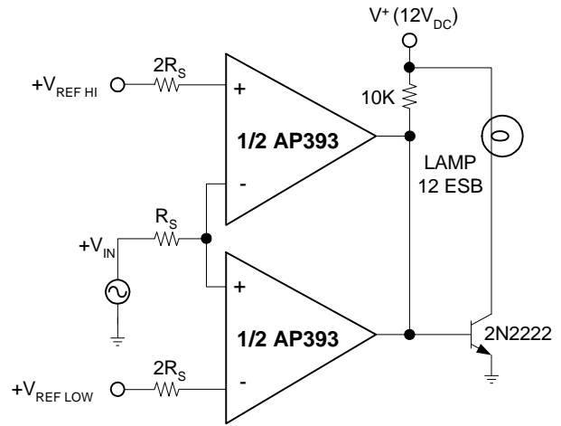
Limit Comparator
