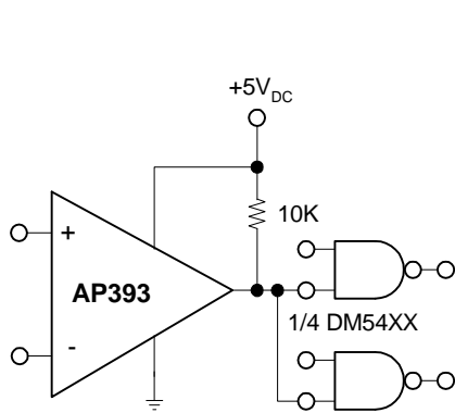
Driving TTL
