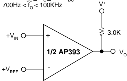
Basic Comparator
